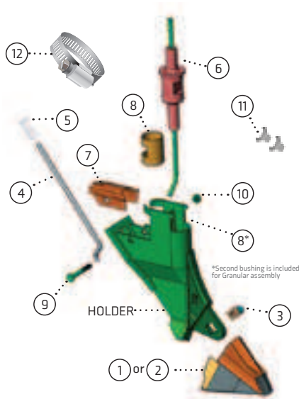
612-ASY-0711 (LEFT) 612-ASY-0712 (RIGHT SHOWN)
